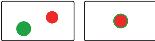
Fig. 12: Aiming using the sight (red: red dot, green: target laser) Left image: Target laser and red dot detectable in sight Right image: Target laser and red dot overlapping
